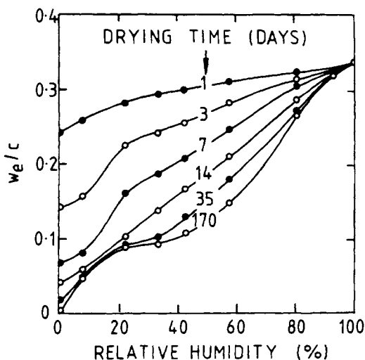
Fig. 8.6 Desorption curves for an initially saturated C_3S paste of w/c ratio 0.5, hydrated for 5.8 years at 25^\circ\text{C} in the form of slab samples 1 mm thick. Each point represents the result of a separate experiment in which the sample was exposed to an atmosphere of given relative humidity for the drying time shown. After G75.
