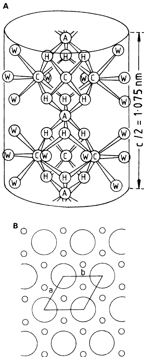
Fig. 6.4 Crystal structure of ettringite. (A) Part of a single column in (11\bar{2}0) projection; A = Al, C = Ca, H = O of an OH group, W = O of an \text{H}_2\text{O} molecule. Hydrogen atoms are omitted, as are the \text{H}_2\text{O} molecules attached to those calcium atoms lying in the central vertical line of the figure. (B) Projection on the ab -plane, showing columns (large circles) and channels (small circles); the unit cell, with a \approx 1.123 \text{ nm} , is outlined. Modified from S70.
