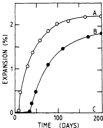
Fig. 12.6 Typical relations between expansion produced by ASR and age; data are for mortars with w/c=0.41 and aggregate/cement = 2, (A) with 6.7% of Beltane opal in the aggregate and a cement with Na_2O_e=1.24\% , and (B) with 4.5% of Beltane opal in the aggregate and Na_2O_e=0.8\% . After H76.
