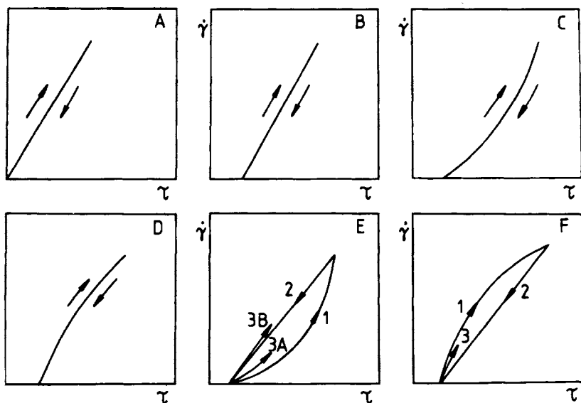
Fig. 8.1 Idealized plots of shear rate \dot{\gamma} against shear stress \tau for fluids of various types. (A) Newtonian fluid. (B) Bingham fluid. (C) Shear thinning. (D) Shear thickening. (E) Positive hysteresis: 1, 2, 3A thixotropy; 1, 2, 3B rheodestruction. (F) Negative hysteresis with antithixotropy.
