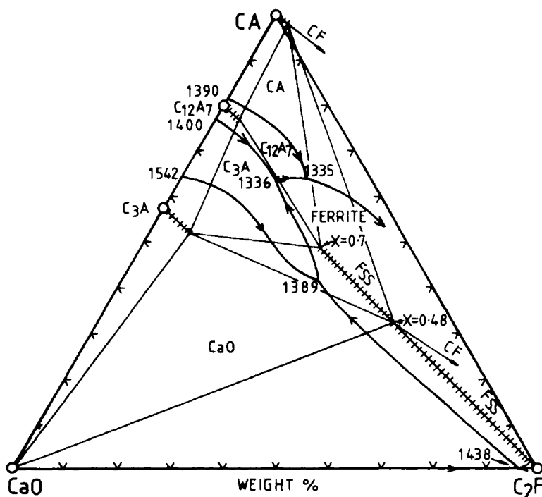
Fig. 2.5 Part of the system \text{CaO-Al}_2\text{O}_3\text{-Fe}_2\text{O}_3 . Hatched lines indicate solid solutions. Ferrite phase compositions are indicated by the quantity x , which relates to the formula \text{Ca}_2(\text{Al}_x\text{Fe}_{1-x})_2\text{O}_5 . After N9 and M27.
