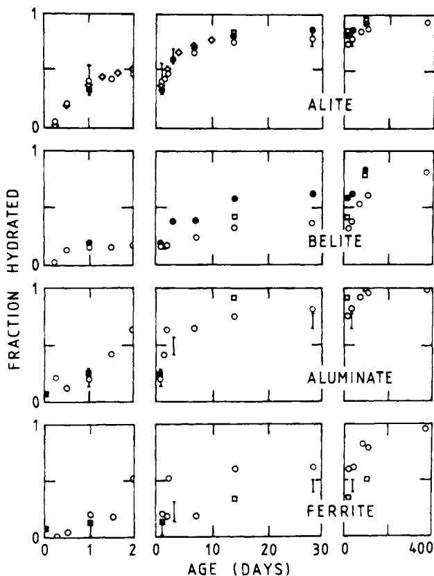
Fig. 7.4 QXDA results for the fractions of the clinker phases reacted in Portland cement pastes. Solid circles: C46, w/c = 0.65 . Diamonds: B112, sample C2. Vertical lines: O9, range for 7 samples. Open circles: D15. Open squares: P33, samples cured at 100% RH. Solid squares: T35, clinker interground with gypsum.
