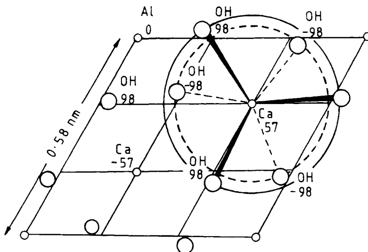
Fig. 6.1 Structure of a single principal layer of composition [\text{Ca}_2\text{Al}(\text{OH})_6]^+ in an AFm phase, in ab -projection. Distances of calcium, aluminium and oxygen atoms above or below the central plane of the layer are in pm. Hydrogen atoms are not shown. Large circles illustrate the distortion of the \text{CaO}_6 octahedra, which allows the coordination of each calcium atom to rise to 7 through the addition of a water molecule (not shown) directly above or below it in this projection.
