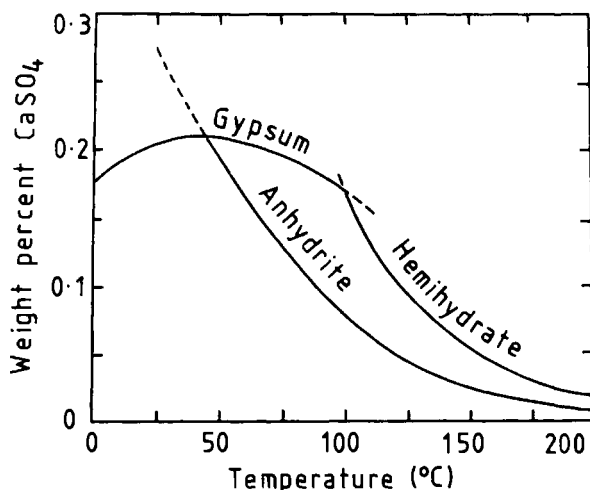
Fig. 6.5 The \text{CaSO}_4\text{-H}_2\text{O} system. After P29.
