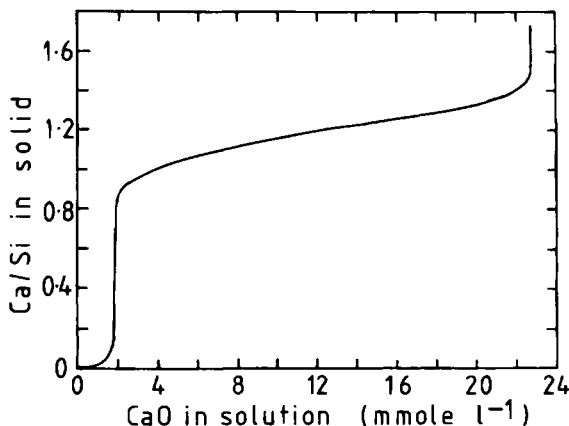
Fig. 5.11 Metastable equilibrium curve relating the \text{Ca/Si} ratios of \text{C-S-H} preparations to the analytical concentration of \text{CaO} in the solution, selected as typical from the results of many investigations. After S60.
