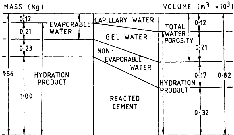
Fig. 8.3 Illustration of the Powers-Brown yard description of a fully hydrated and saturated Portland cement paste of initial water/cement ratio 0.5. All quantities refer to 1 kg of cement.
