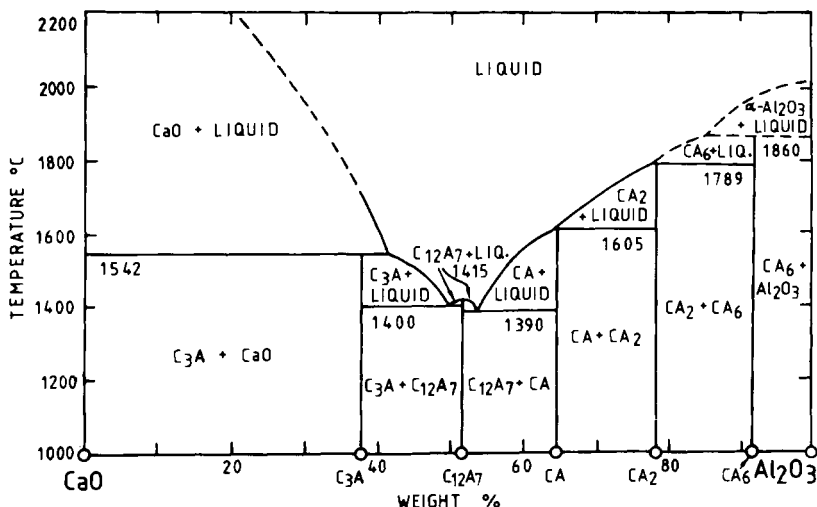
Fig. 2.2 The system \text{CaO}-\text{Al}_2\text{O}_3 modified by the presence of small amounts of \text{H}_2\text{O} and \text{O}_2 , and thus representing the behaviour in air of ordinary humidity. After R4, with later modifications (C5,N6,N7).
