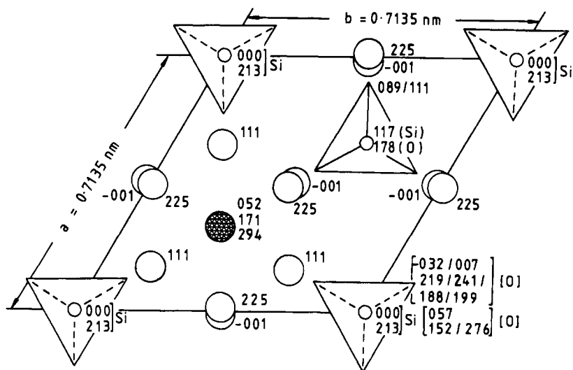
Fig. 1.1 Crystal structure of the R -modification of C_3S , based on the results of Nishi and Takéuchi (N2) and showing Ca atoms (large open circles), Si atoms (small open circles), oxide ions (large hatched circle) and oxygen tetrahedra (triangles). Heights of atoms are in thousandths of the cell height ( c = 2.5586 nm), slashes denoting statistical alternatives. Oxygen tetrahedra are shown in averaged orientations; in reality, each is tilted around its enclosed Si atom statistically in any one of three directions so as to preserve the threefold symmetry. All tetrahedra point upwards excepting those surrounding the Si atoms at height 213, of which 70% point downwards and 30% upwards. Only the bottom third of the cell is shown, the middle and top thirds being derivable from it by translations of 1/3 , 2/3 , 1/3 and 2/3 , 1/3 , 2/3 parallel to the a , b and c axes respectively.
