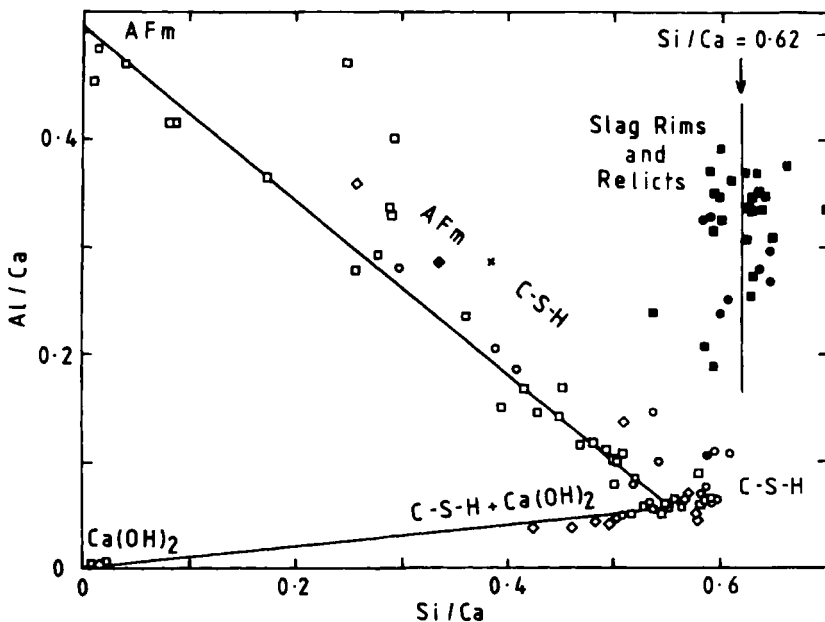
Fig. 9.1 Si/Ca and Al/Ca atom ratios from individual X-ray microanalyses of a slag cement paste (40% slag; w/s = 0.5) hydrated for various times at 25°C. Mg/Si < 0.15: ◇, 28 days; □, 6 months; ○, 14 months. Mg/Si ≥ 0.15: ◆, 28 days, ■, 6 months; ●, 14 months. From H58.
