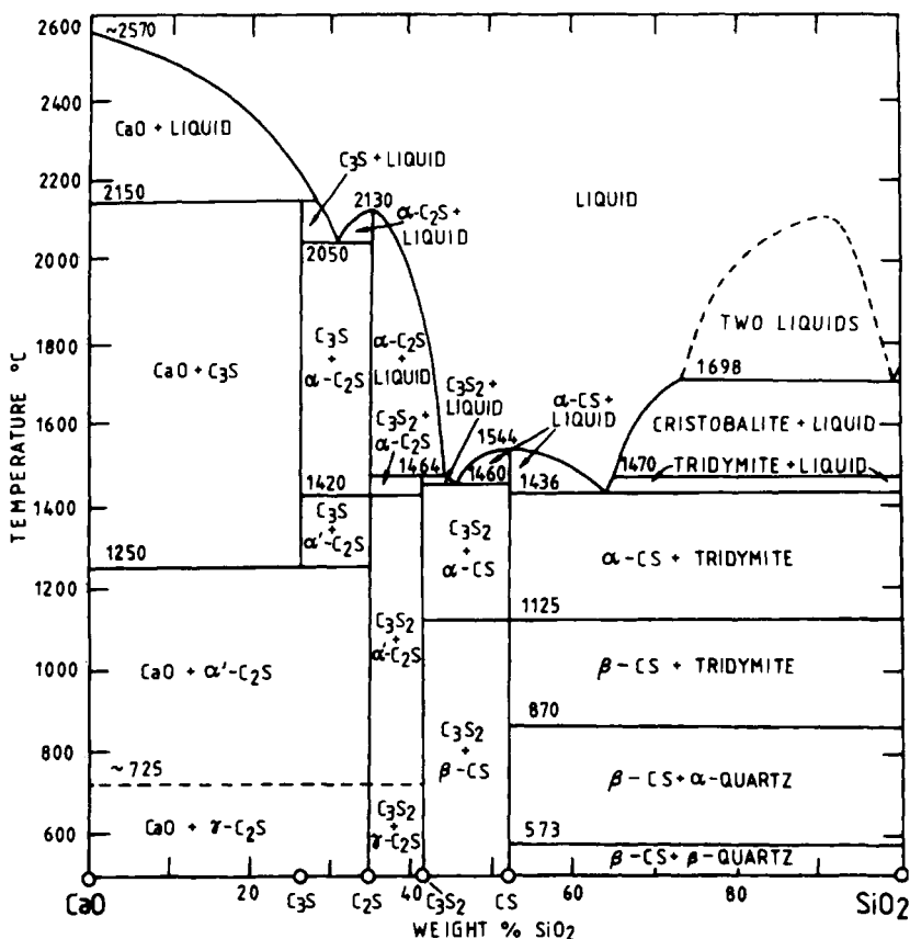
Fig. 2.1 The system \text{CaO-SiO}_2 . After D2, with later modifications (G12,O3, R4,W2).
