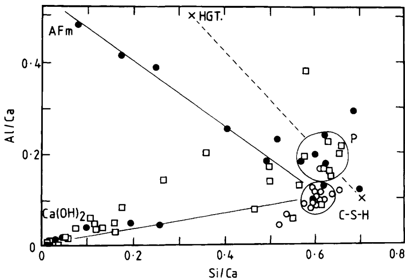
Fig. 9.5 Si/Ca and Al/Ca atom ratios from individual X-ray microanalyses of a 91-day-old paste of a Portland-flyash cement (28% of a flyash low in CaO; w/s=0.5 ). Open circles, inner product from alite or belite; open squares, regions near to flyash particles, and sometimes also to CH; solid circles, undesignated product. P: suggested composition of inner product from flyash, possibly consisting largely of C-S-H and hydrogarnet (HGT). Modified from H4.
